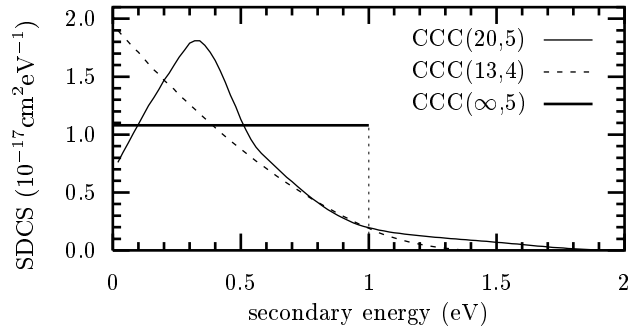
Figure 1. The singly differential cross sections arising in the \text{CCC}(N_0, l_{\max}) (see text) calculations. The step function labeled by \text{CCC}(\infty, 5) is an integral preserving estimate.
